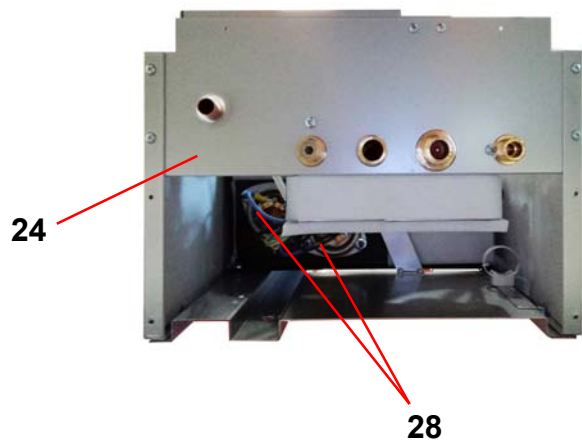
Detail view: Body / Heating Elements
