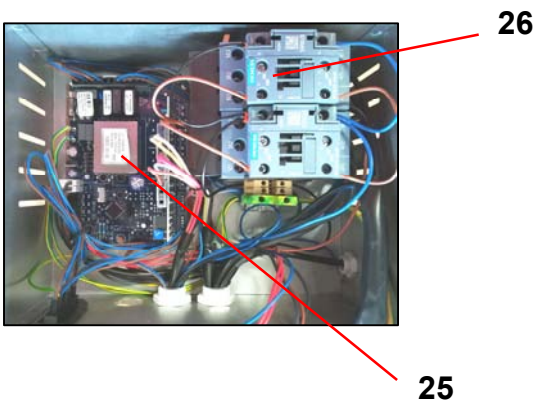
4 Detail view: Electric Box
